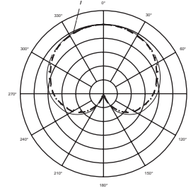
Polar Pattern
