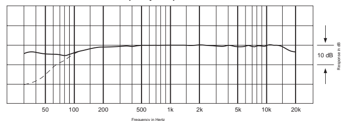
Frequency Response
